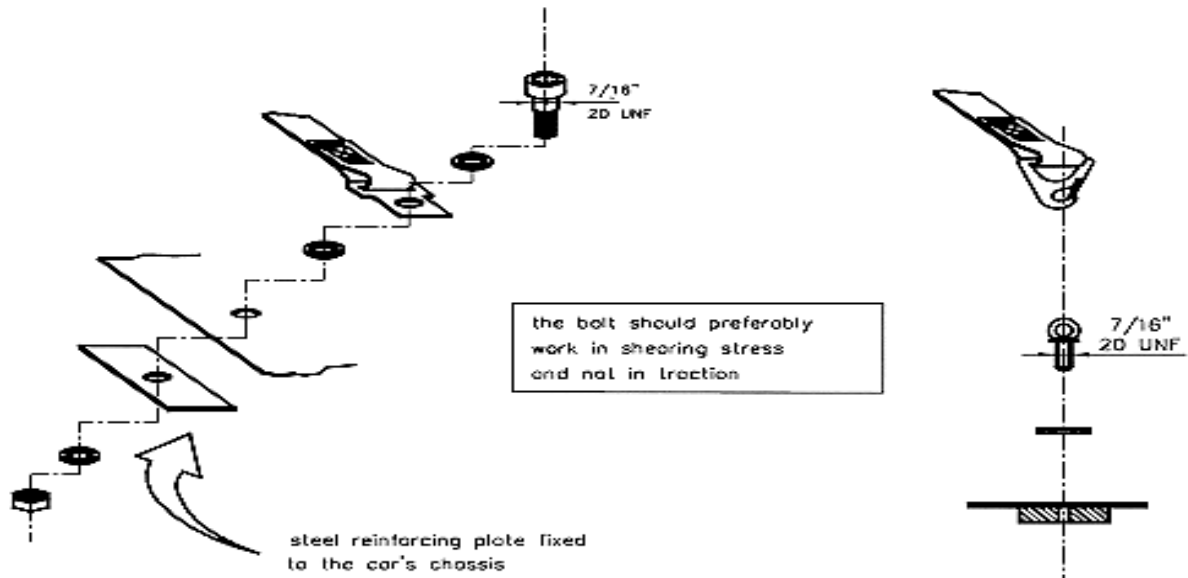
Drawing No 253-43
